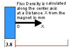
Fig. 4 - Flux density geometry for a 15.25cm diameter grade N38 permanent magnet. Courtesy of International Magnetic Solutions.
