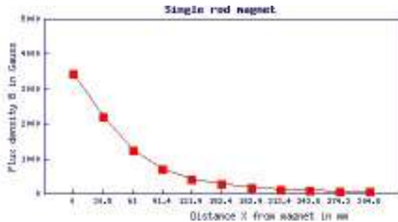
Fig. 3 - Flux density decreases with the inverse cube of the distance from the magnet surface. Courtesy of International Magnetic Solutions.
